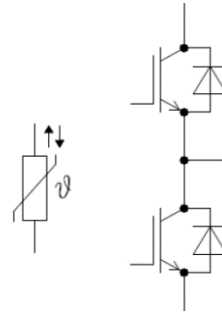
Equivalent Circuit Schematic
